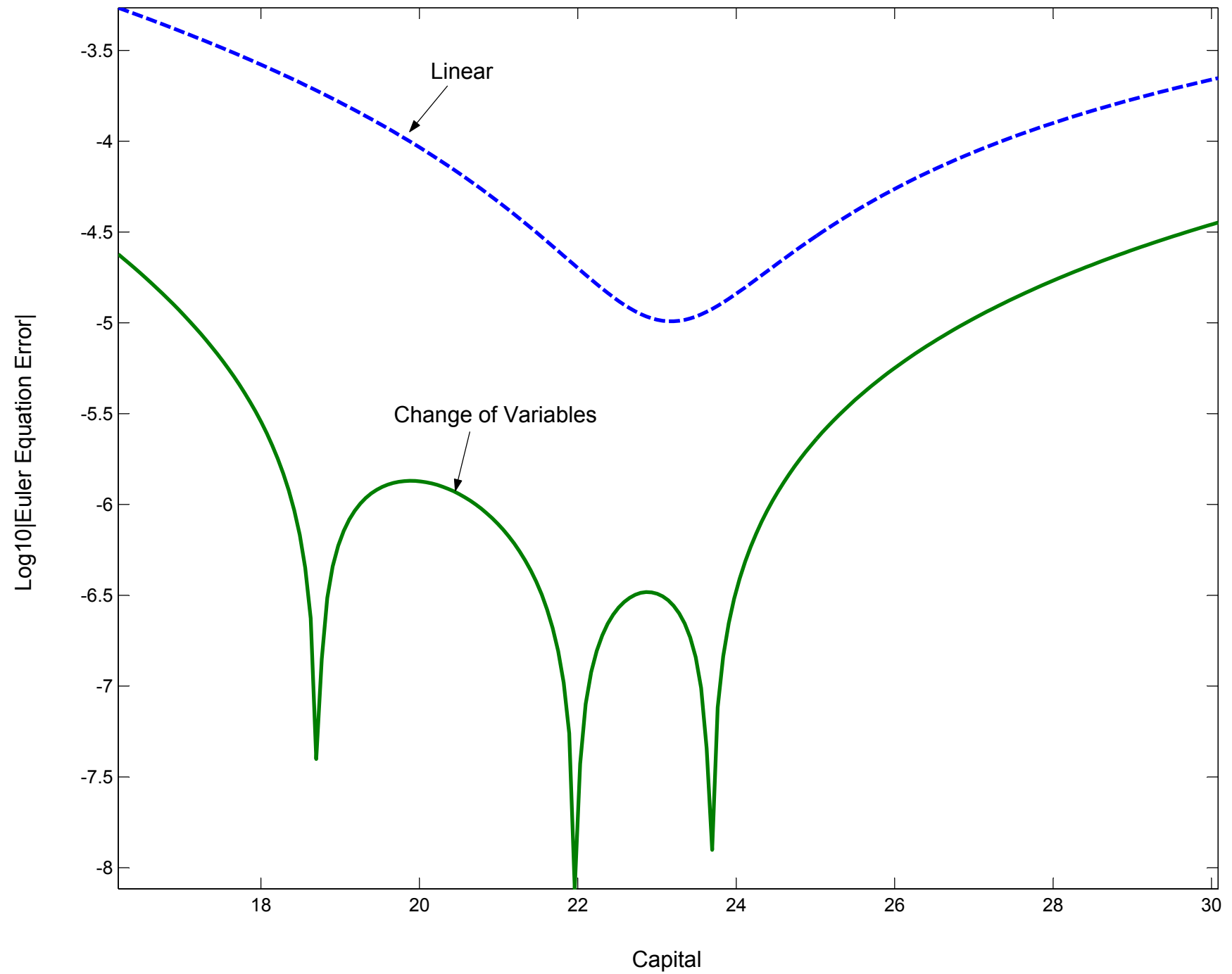
Figure 1: Euler Equation Errors at z = 0 , \tau = 2 / \sigma = 0.007
