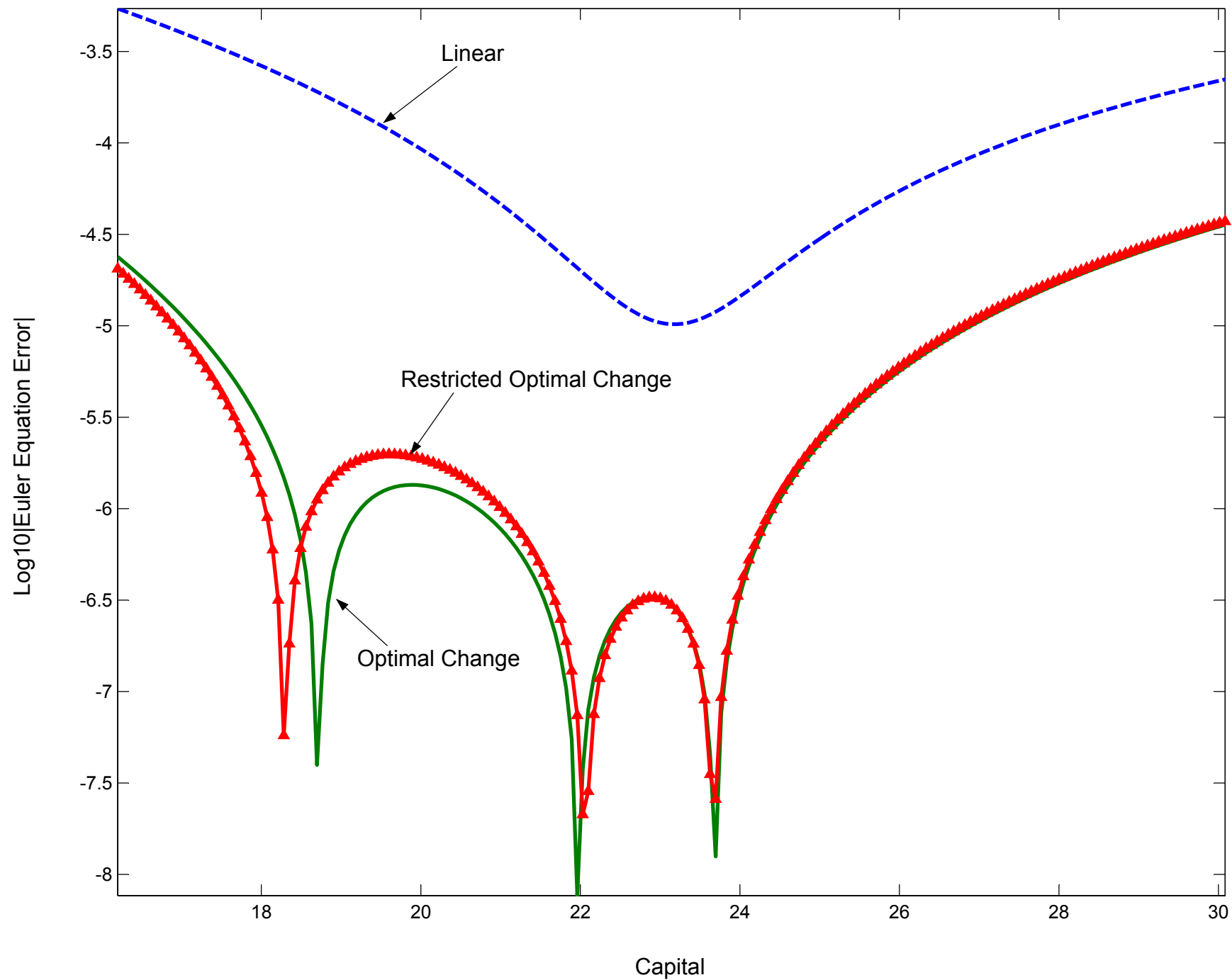
Figure 4: Euler Equation Errors at z = 0 , \tau = 2 / \sigma = 0.007
