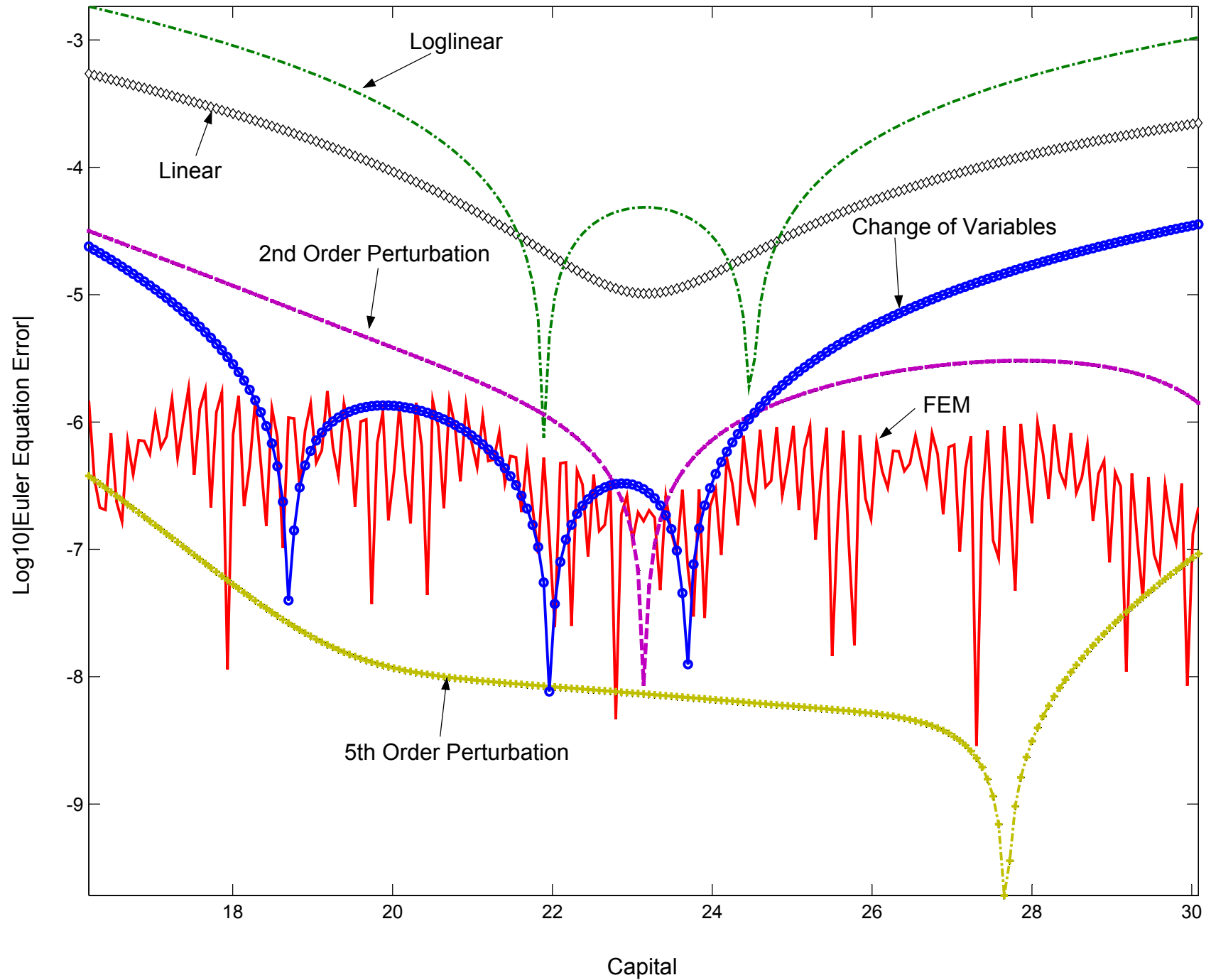
Figure 2 : Euler Equation Errors at z = 0 , \tau = 2 / \sigma = 0.007
