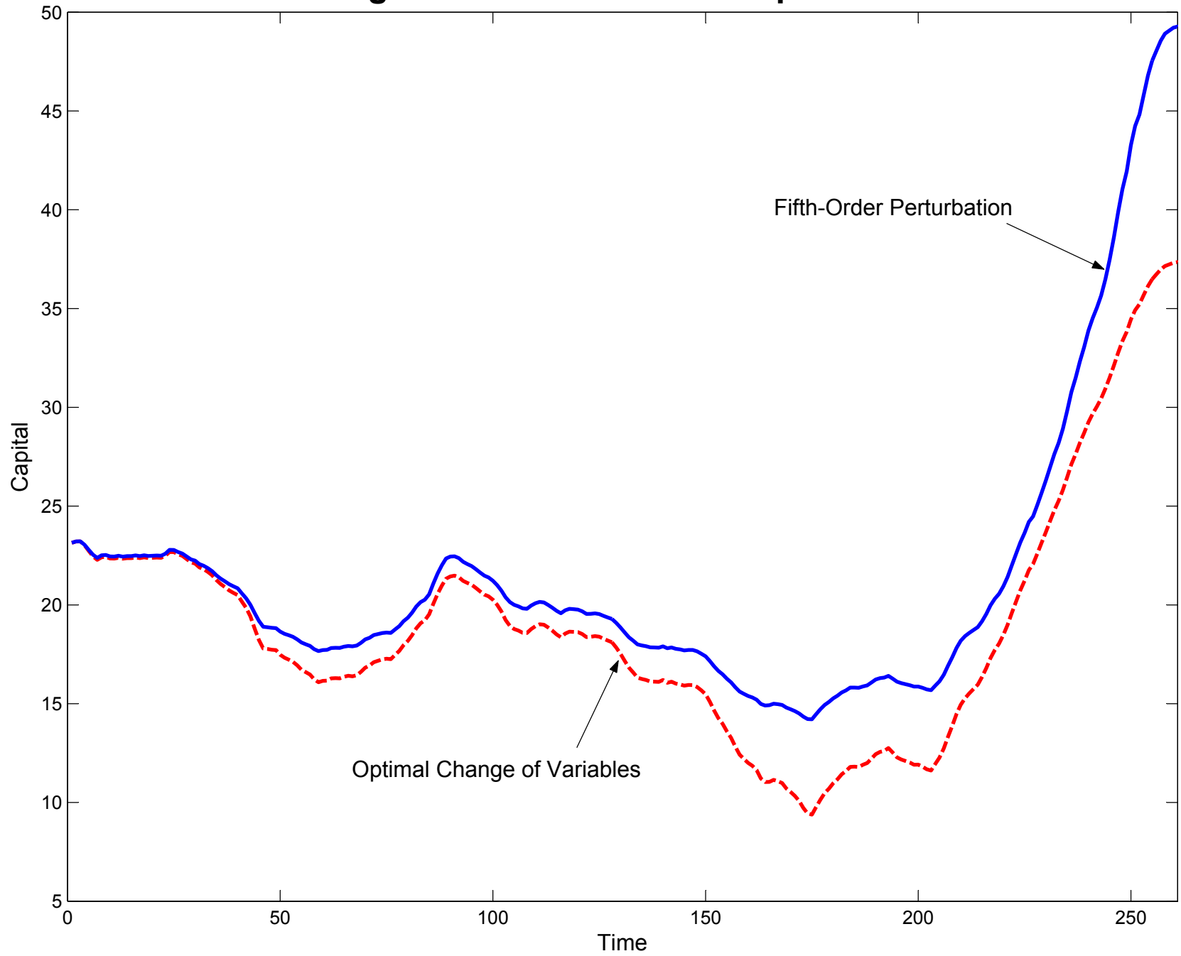
Figure 3: Time Series of Capital
