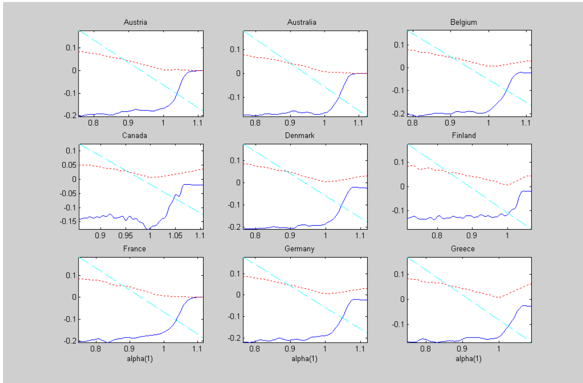
Demeaned estimation for Austria, Australia, Belgium, Canada, Denmark and Finland.
