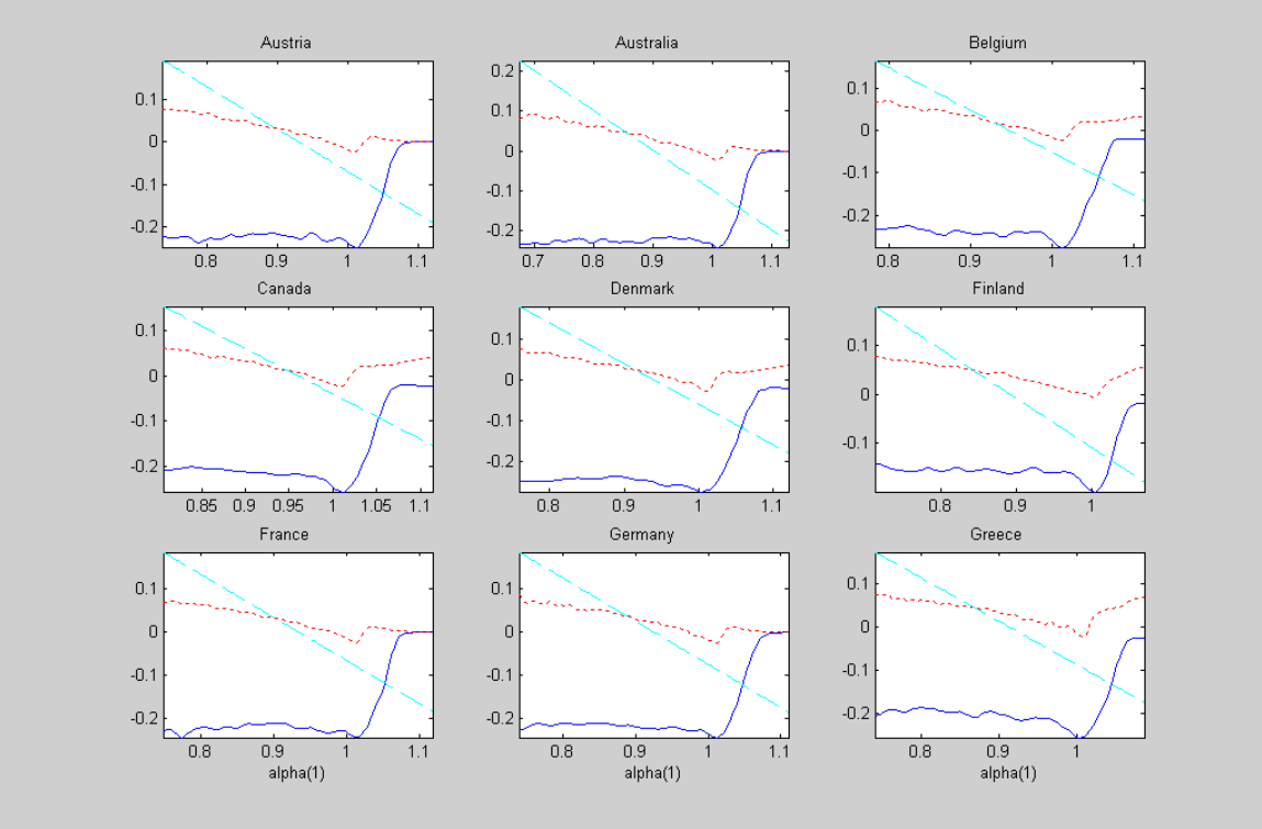
Detrended estimation for Austria, Australia, Belgium, Canada, Denmark and Finland.
