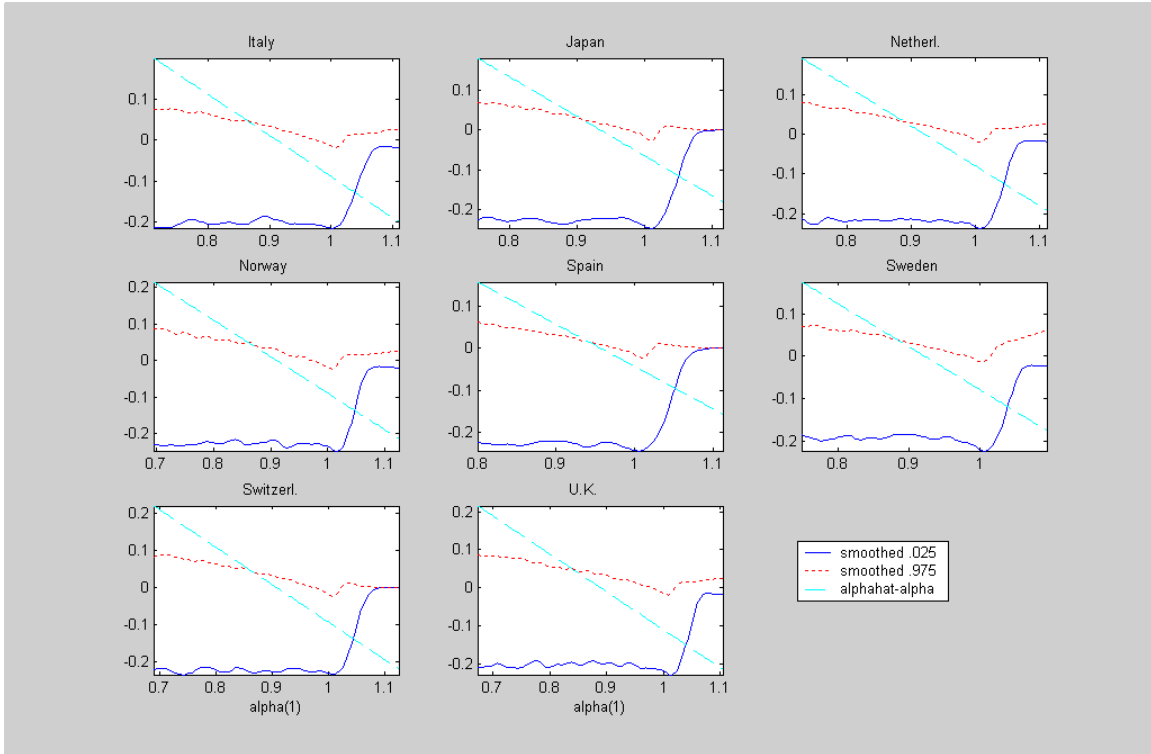
Detrended estimation for Italy, Japan, Netherlands, Norway, Spain, Sweden, Switzerland and U.K.
