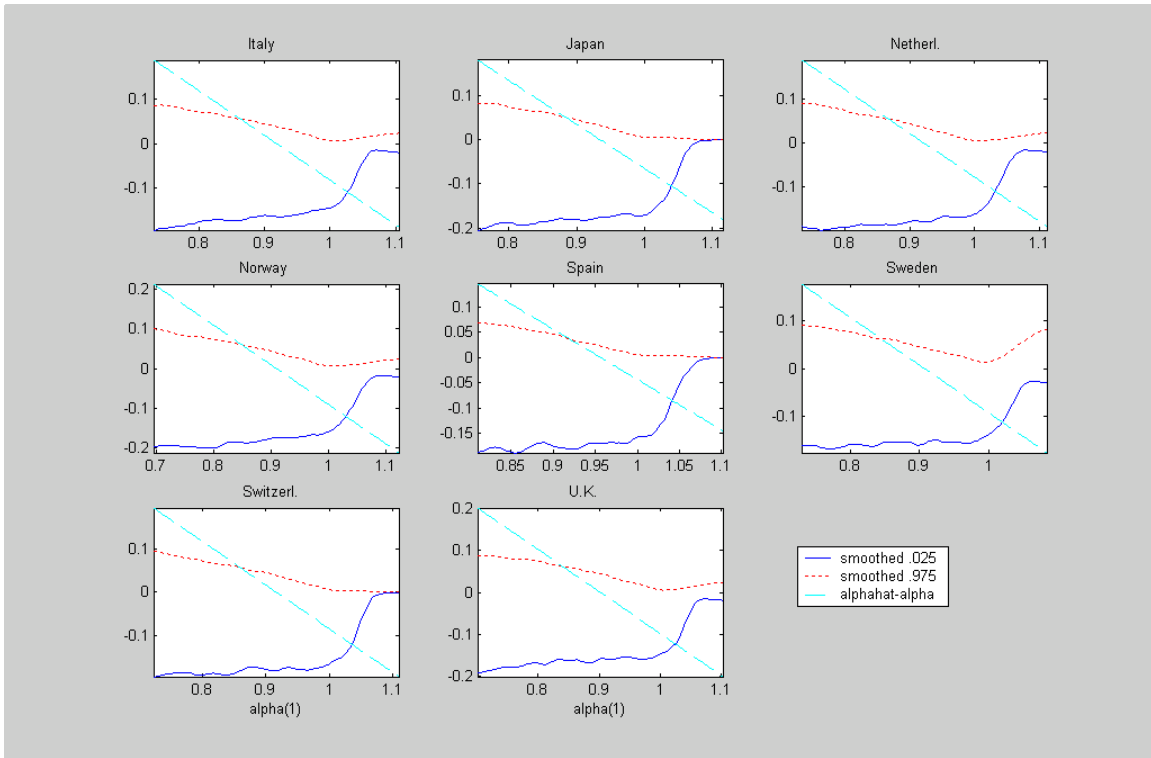
Demeaned estimation for Italy, Japan, Netherlands, Norway, Spain, Sweden, Switzerland and U.K.
