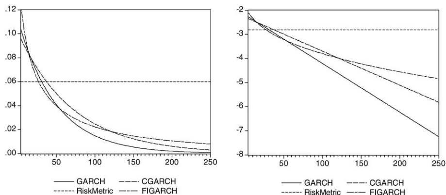
Figure 6. Volatility impulse response coefficients. The left panel graphs the volatility impulse response function, \partial \sigma_{t+h|t}^2 / \partial \varepsilon_t^2 , h = 1, 2, \dots, 250 , for the RiskMetrics forecasts, the standard GARCH(1, 1) model in (3.6), the FIGARCH(1, d , 1) model in (3.18), and the component GARCH model in (3.21) and (3.22). The right panel plots the corresponding logarithmic values.
