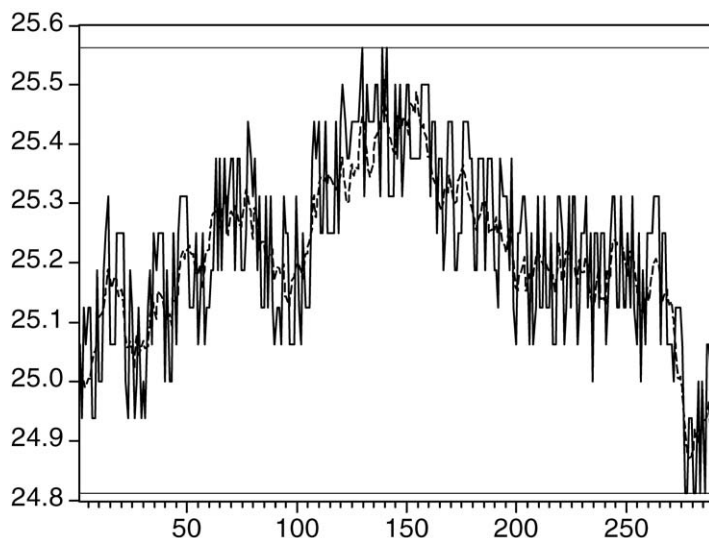
Figure 7. Simulated fundamental and observed intraday prices. The smooth dashed line represents the fundamental, but unobserved, simulated asset price. The jagged solid line solid represents the observed transaction prices reflecting bid or ask driven transactions. The two horizontal lines denote the min and max prices observed within the day.
