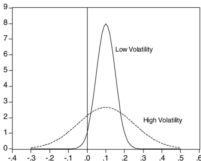
Figure 2. Density forecasts on high volatility and low volatility days. The figure shows two hypothetical return distributions for a low volatility (solid line) and high volatility (dashed line) day. The areas to the left of the vertical line represent the probability of a negative return.
