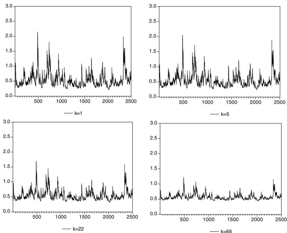
Figure 5. GARCH volatility forecasts and horizons. The four panels show the standardized “daily” GARCH(1, 1) volatility forecasts, k^{-1}\sigma_{t:t+k|t}^2 , for horizons k = 1, 5, 22, 66 .
