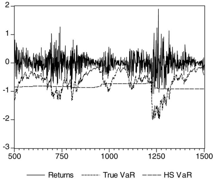
Figure 3. Simulated portfolio returns with dynamic volatility and historical simulation VaRs. The solid line shows a time series of typical simulated daily portfolio returns. The short-dashed line depicts the true one-day-ahead, 1% VaR. The long-dashed line gives the 1% VaR based on the so-called Historical Simulation (HS) technique and a 500-day moving window.
