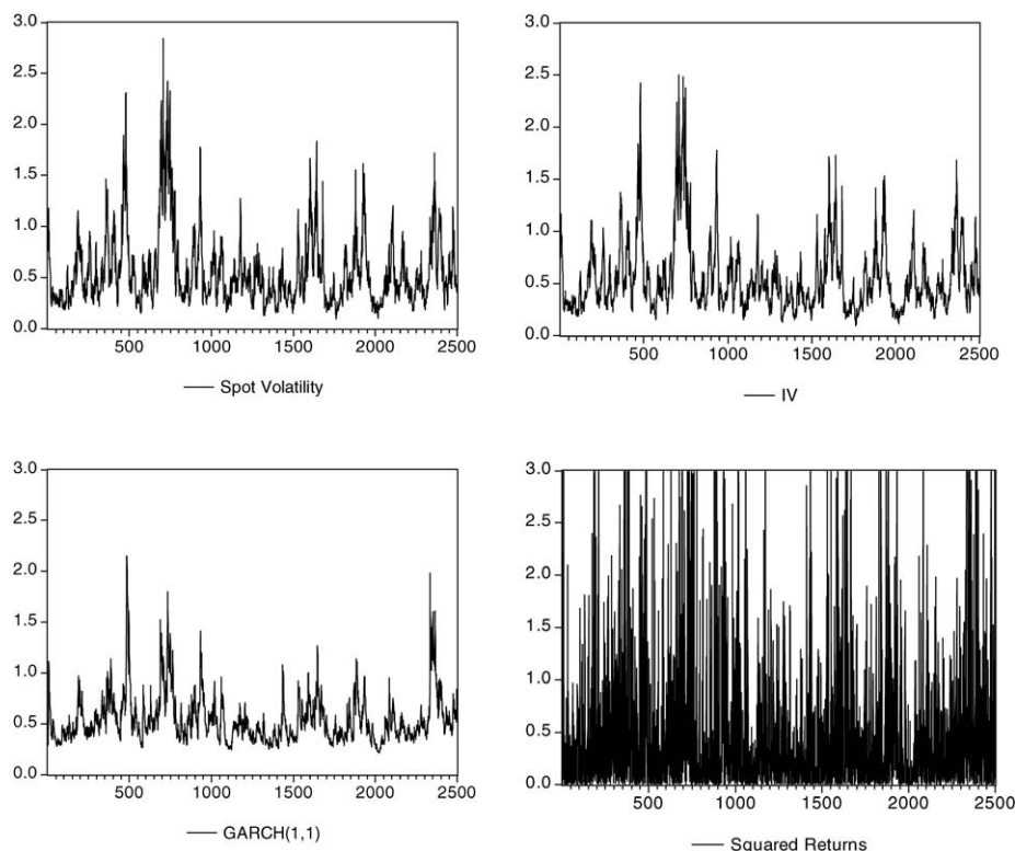
Figure 1. Different volatility concepts. We show the “daily” spot volatility, \sigma^2(t) , the integrated volatility, IV(t) , the discrete-time GARCH based volatility forecasts, \sigma_{t|t-1}^2 , and the corresponding squared returns, r_t^2 , from a simulated continuous-time GARCH diffusion.
