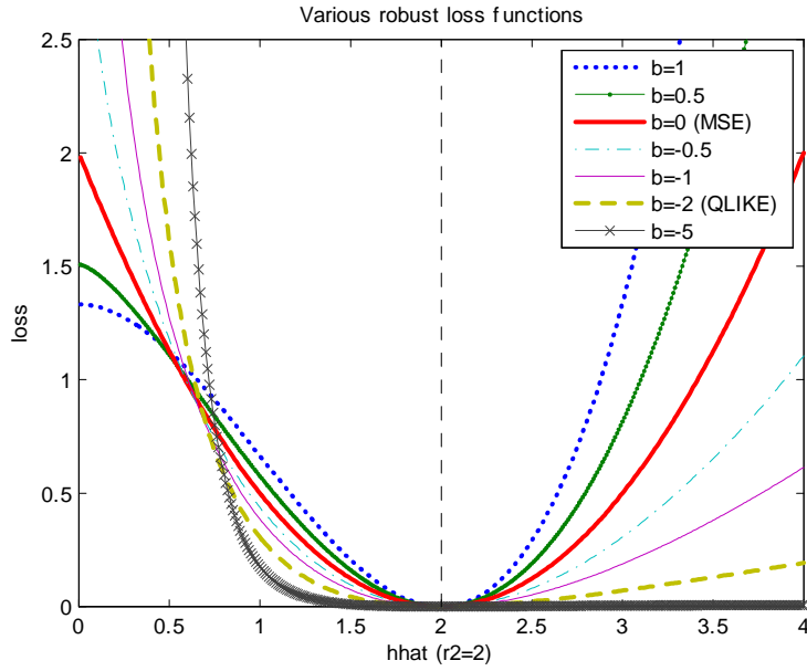
Figure 1: Loss functions for various choices of b . True \sigma^2=2 in this example, with the volatility forecast ranging between 0 and 4. b=0 and b=-2 correspond to the MSE and QLIKE loss functions respectively.
