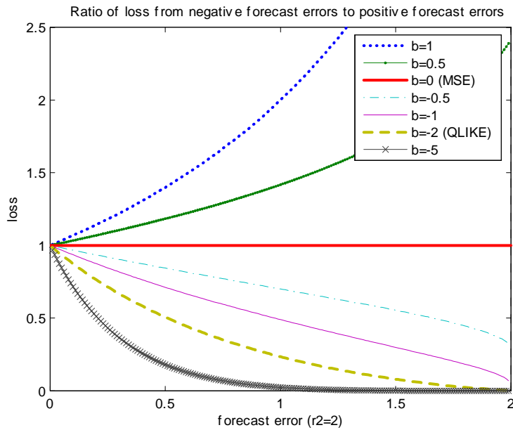
Figure 2: Ratio of losses from negative forecast errors to positive forecast errors, for various choices of b . True \sigma^2=2 in this example, with the volatility forecast ranging between 0 and 4. b=0 and b=-2 correspond to the MSE and QLIKE loss functions respectively.
