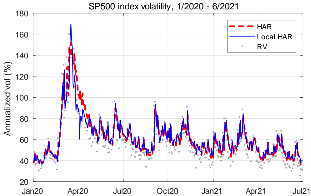
Figure 4: This figure shows the predicted volatility from a HAR model estimated using local or non-local QML, along with realized volatility, over the last 18 months of the sample period.
