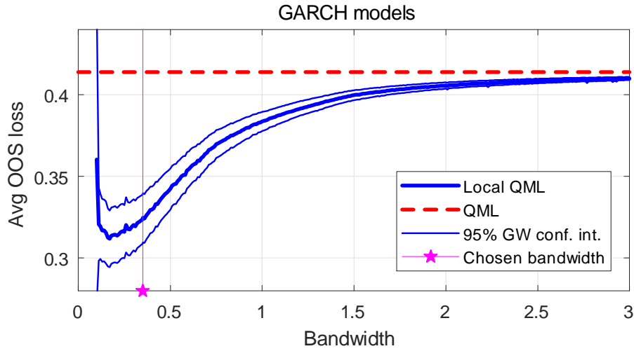
Figure 3: This plot shows the average out-of-sample (OOS) loss using local QML estimates of a GARCH model as a function of the bandwidth. The state variable is realized variance. The dashed line is the (non-local) QML average loss, and the thin solid lines show the 95% GW confidence interval on the difference between local and non-local average loss. The starred vertical line shows the bandwidth chosen based on a validation sample separate from the OOS period.
