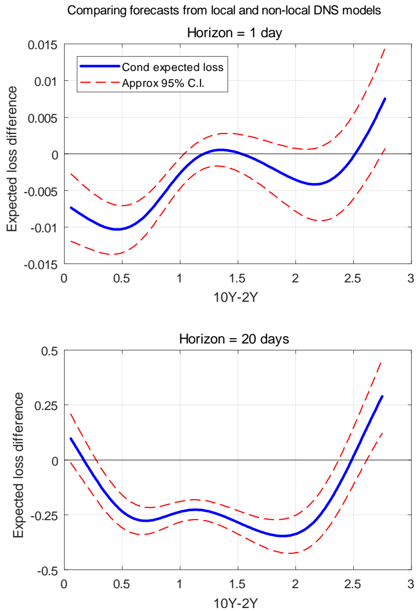
Figure 6: This figure presents estimates of the expected out-of-sample loss difference of a dynamic Nelson-Siegel (DNS) model estimated via local OLS or non-local OLS, both conditional on the difference between 10-year and 2-year government bond yields (10Y-2Y). Positive loss differences indicate the non-local method is preferred.
