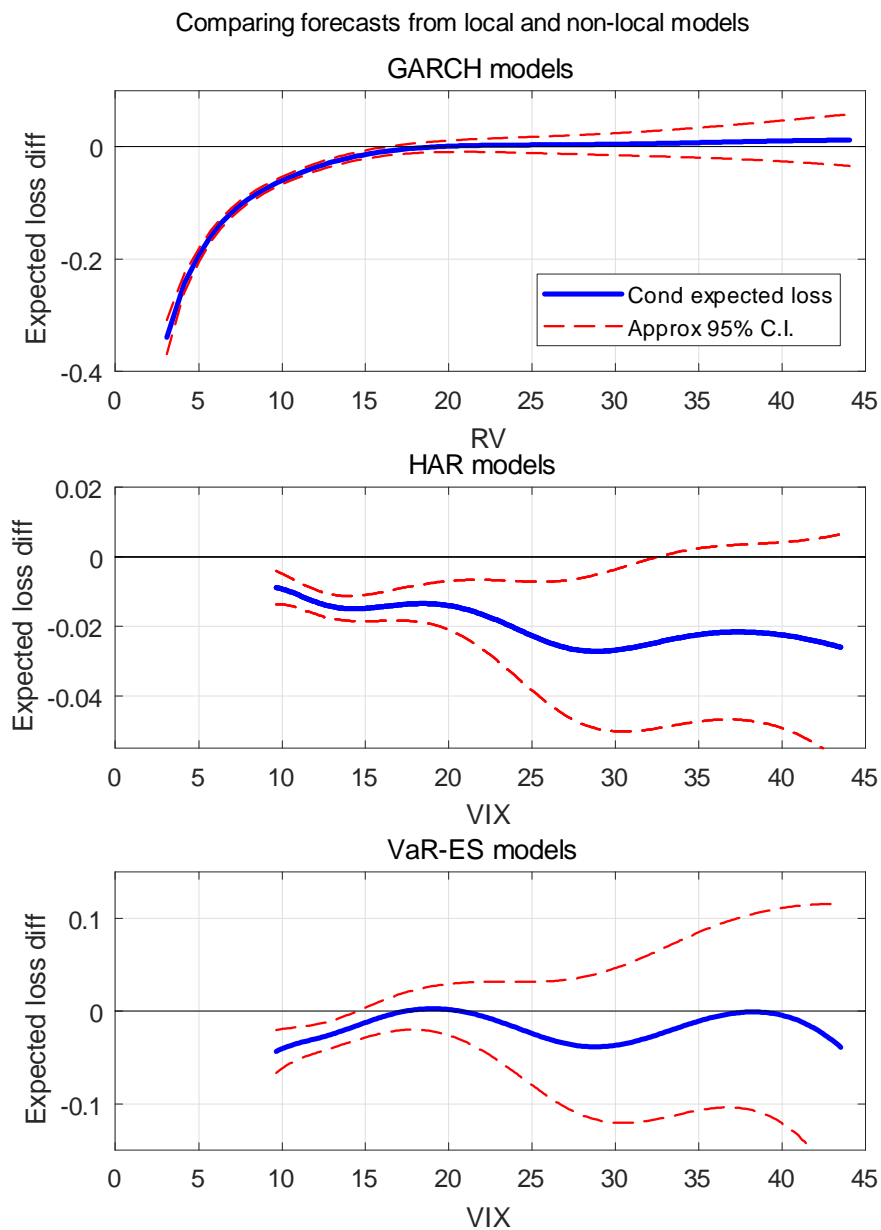
Figure 5: This figure presents estimates of the expected out-of-sample loss differences from models estimated via local or non-local methods, conditional on realized volatility (top panel) or VIX (lower two panels). Positive loss differences indicate the non-local method is preferred.
