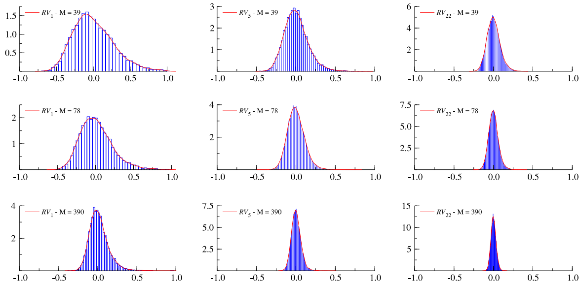
Fig. 1. Estimation error of RV. The figure shows the simulated distribution of RV/IV - 1 . The top, middle and bottom panels show the results for M = 39, 78, and 390, respectively, while the left, middle and right panels show the results for daily, weekly, and monthly forecast horizons, respectively.
