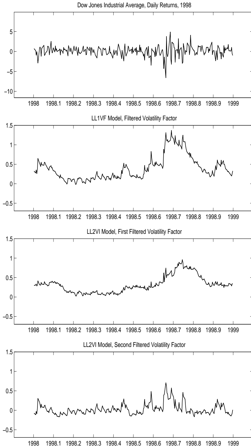
Figure 5: Reprojection of volatility factors from LL1VF and LL2VI Models - 1998
