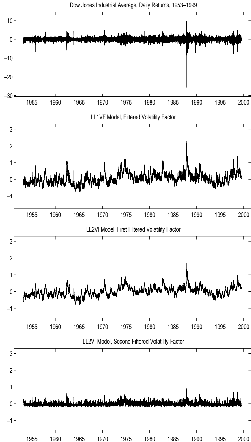
Figure 4: Reprojection of volatility factors from LL1VF and LL2VI Models - 1953-1999
